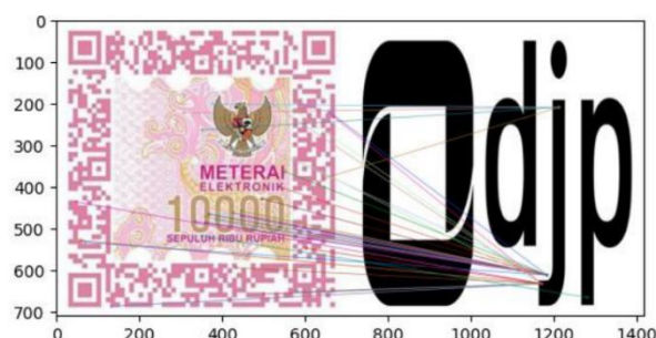
Figure 11 SIFT Watermarking
